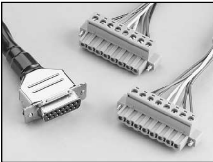
CA-322-1: Dual temperature control cable. For use with: 2510, 8542, 8544
