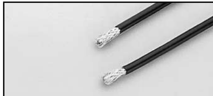
SC-22: Low noise triax cable without connectors (sold by the foot). For use with: CS-141, CS-631
