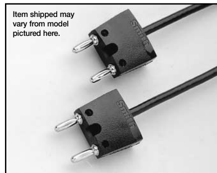
CA-18-1: 1.2m (4 ft) shielded cable terminated with a dual banana plug on each end. For use with binding post inputs or dual banana jacks.
