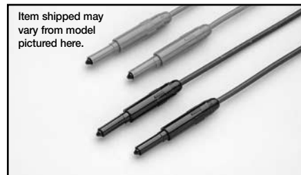
Model 8607 1kV Source Banana Cable Set: The 8607 cable set is made up of one red and one black high voltage test leads with banana plug ends. The cables are 1 meter long and have a voltage rating of 1000V DC or AC peak
